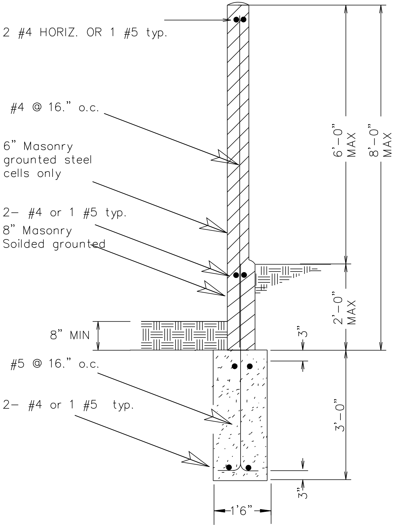
RETAINING WALL
